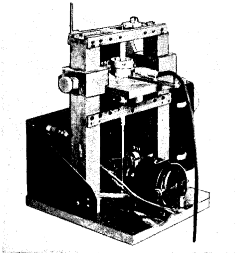
FIG. 18-13.—Rotary-probe setup.
